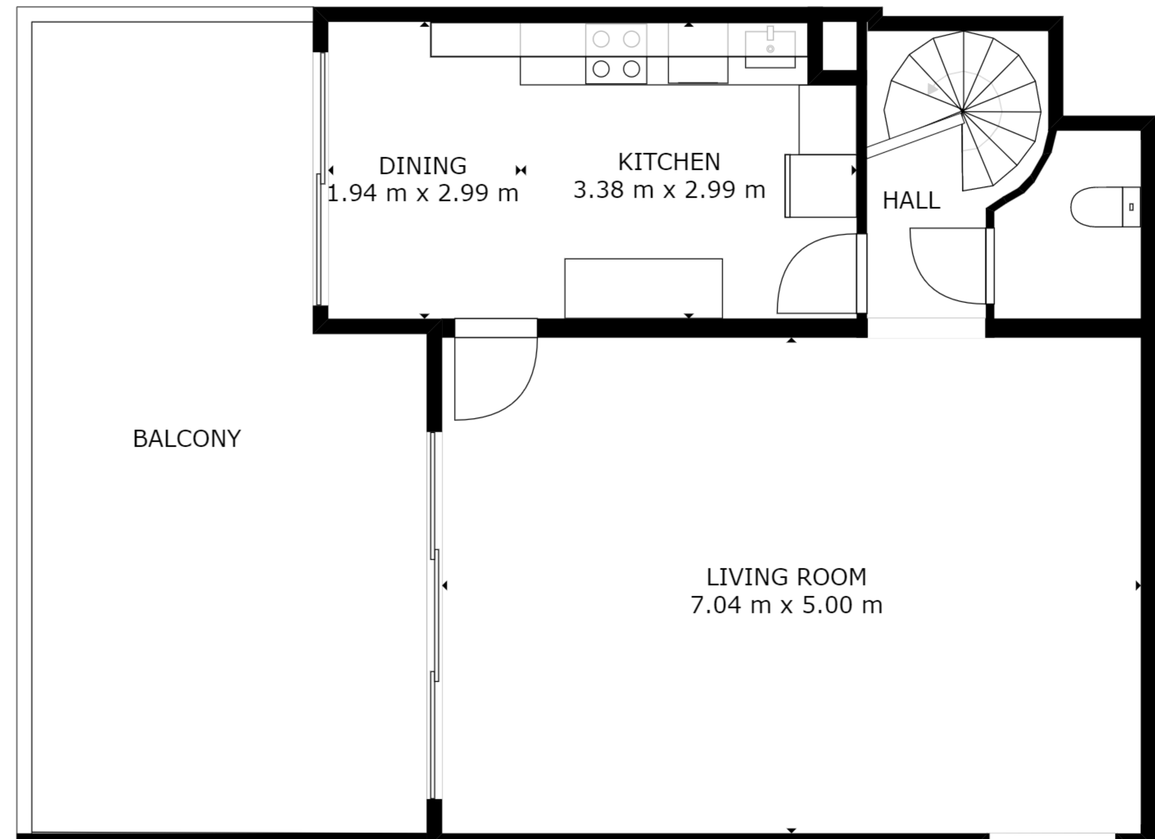
FLOOR 2
